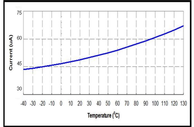
Quiescent Supply Current vs. Temperature
