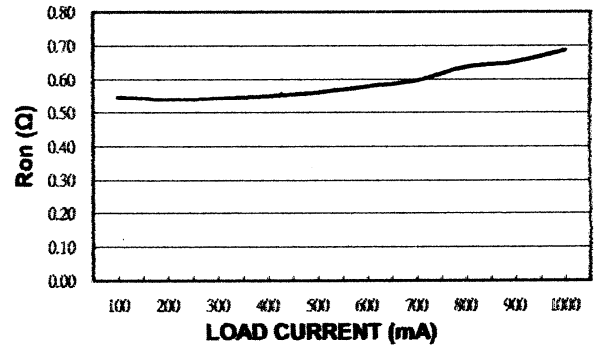
Ron vs. LOAD CURRENT
