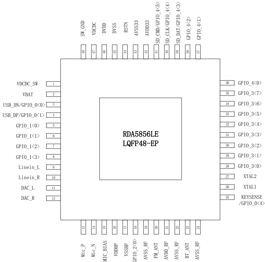
Figure 1 Pin Assignment
