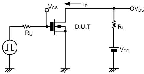
Fig.8 Switching time measurement circuit
