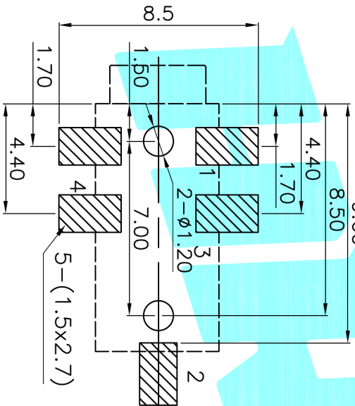
P.C.B LAYOUT(copper-sided view) 9.60
