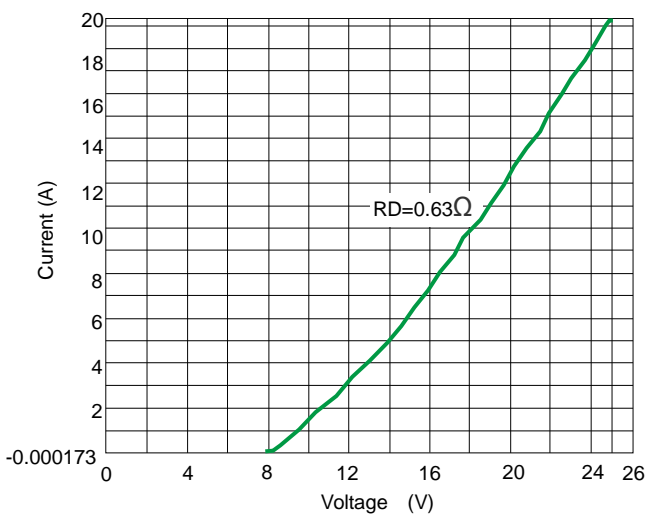
Fig 7. TLP Measurement
