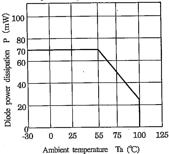
Diode power dissipation vs. ambient temperature
