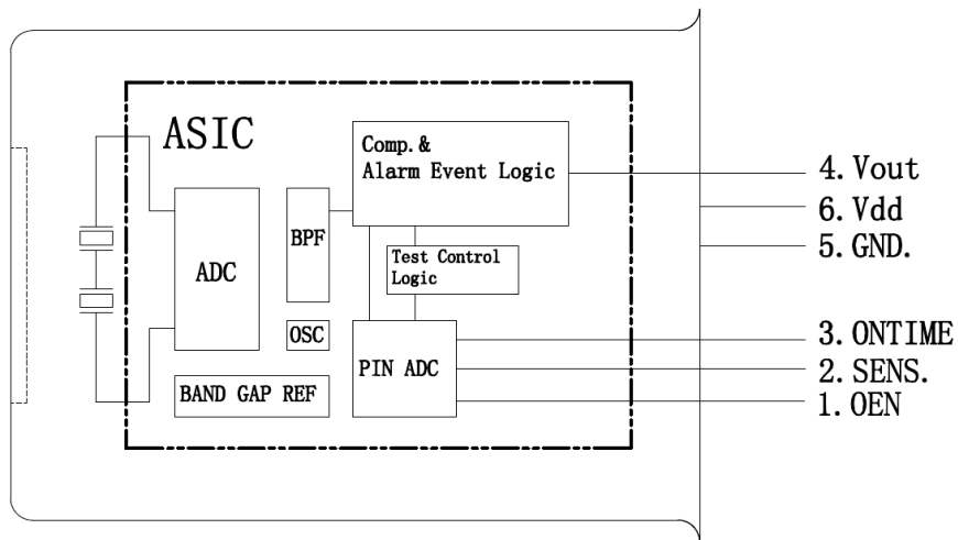
Fig.3: Circuit configuration
