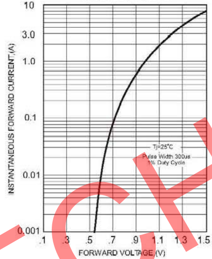
FIG.2-TYPICAL FORWARD CHARACTERISTICS
