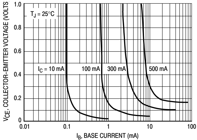
Figure 5. Saturation Region
