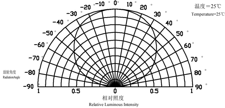
Radiation Diagram
