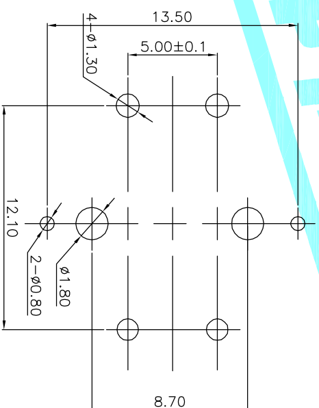
PCBLAYOUT(pattern Side)
