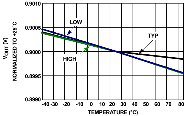
FIGURE 6. V_{OUT} vs TEMPERATURE NORMALIZED to +25^\circ C
