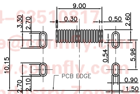
RECOMMEND P.C.B LAYORT (Tolerance ±0.05)
