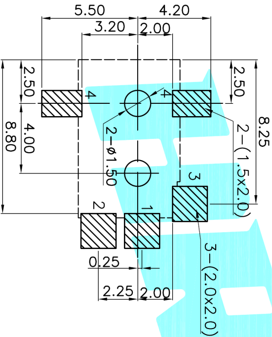
P.C.B LAYOUT(Copper-side view)
