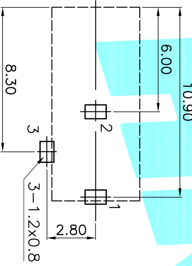
P.C.B LAYOUT(Copper-side view)
