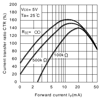
Fig.5 Current Transfer Ratio vs. Forward Current
