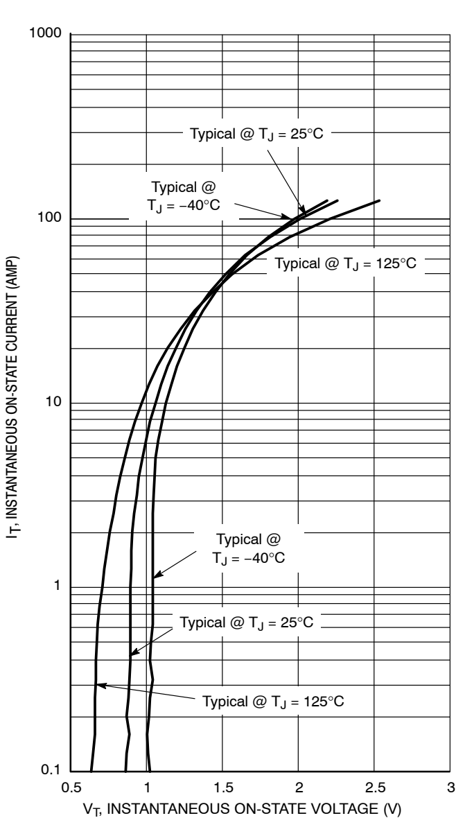
Figure 3. On-State Characteristics
