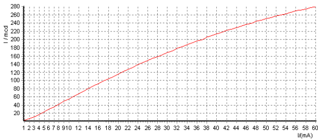
电流-光强曲线 Current-Luminous intensity Curve
