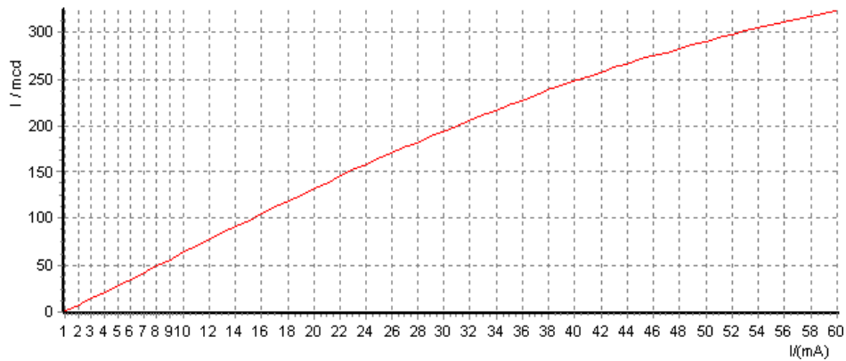
电流-光强曲线 Current-Luminous intensity Curve
